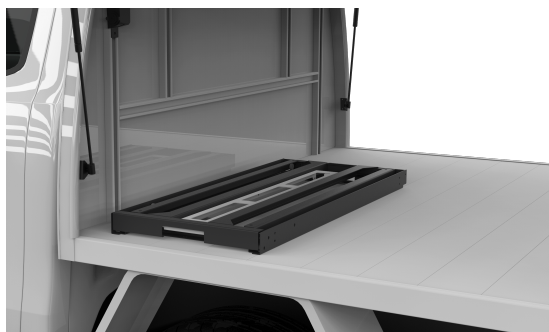
ONE-CLICK MEDIUM DUTY SLIDES W460 x L640mm
