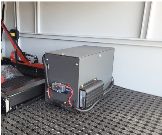
BATTERY BOXES L810 x W240 x H315mm
