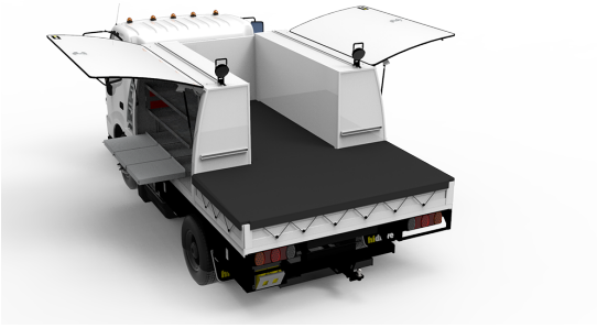
LOAD COVERS (TRUCK) Rear Tray & Aisle (above)
